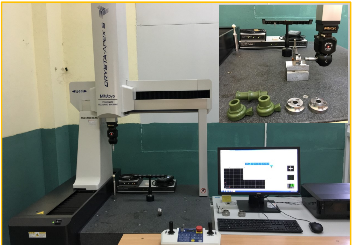
COORDINATE MEASUREMENT MACHINE (CMM)
